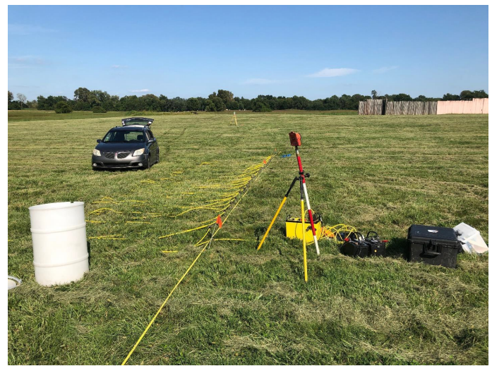
ERT in the Ramey field at Cahokia. Note the palisade wall reconstruction in the background.
